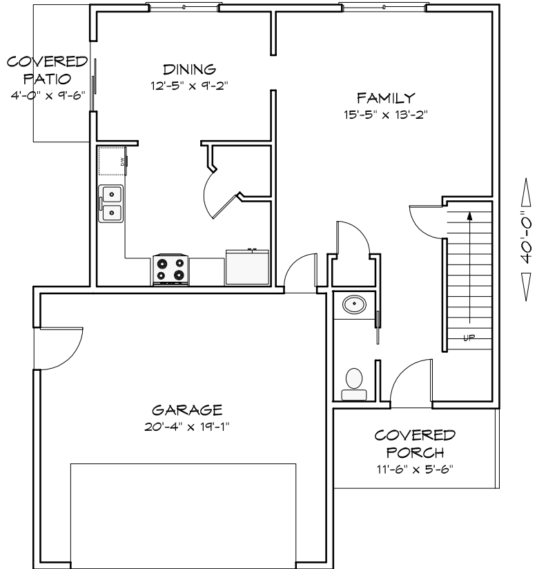
MAIN FLOOR 686 SQUARE FEET
