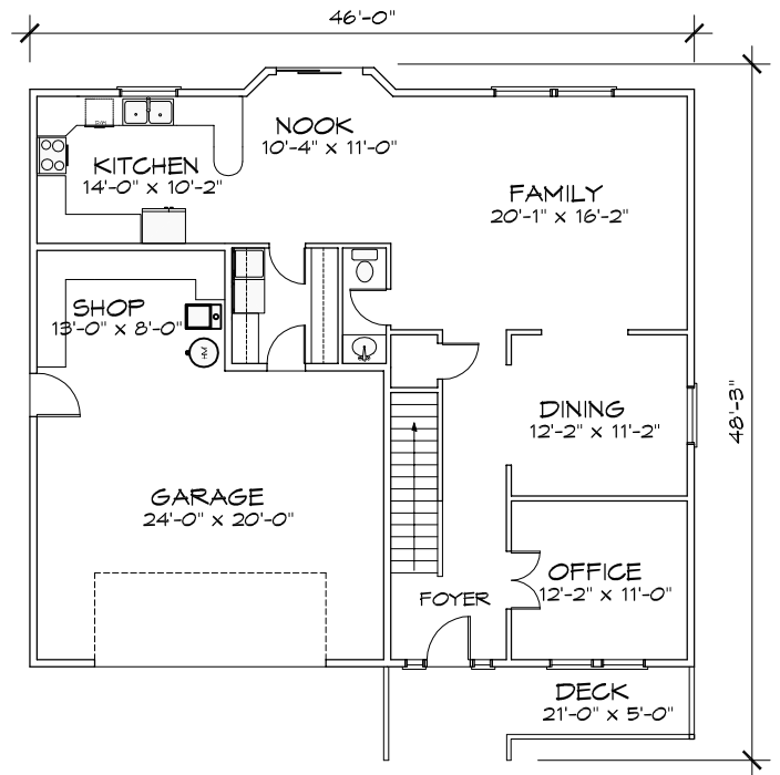
MAIN FLOOR 1220 SQUARE FEET
