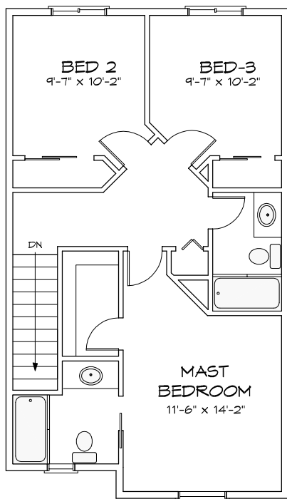
UPPER FLOOR 670 SQUARE FEET
