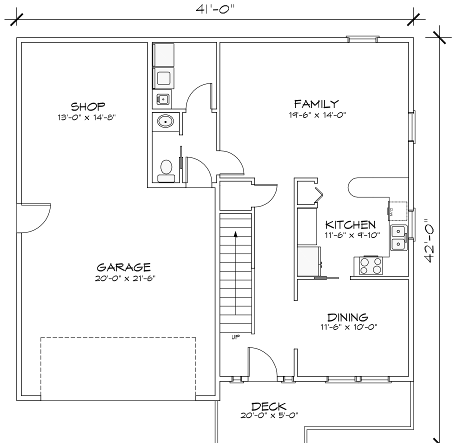
MAIN FLOOR 825 SQUARE FEET
